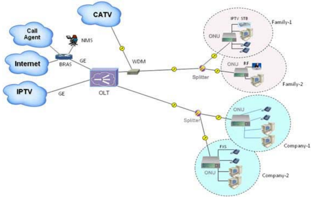
Figure: OP151 Application Diagram
